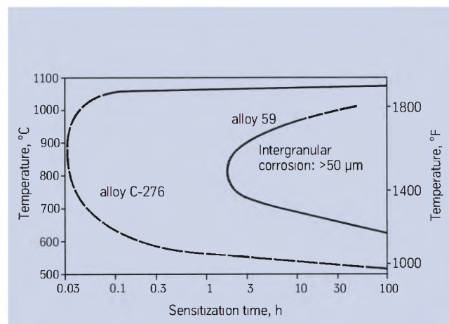
Fig. 1 – Time-temperature-sensitization (TTS) diagram for Nicrofer 5716 hMoW and Nicrofer 5923 hMo according to the Streicher test (ASTM G-28, Method A).
