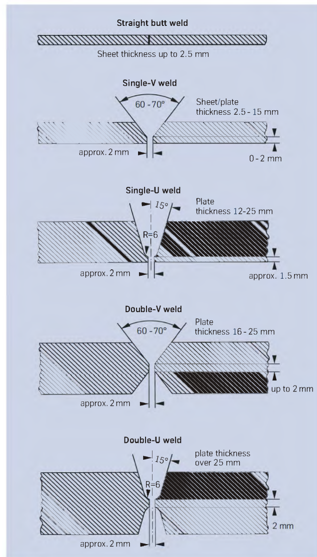
Fig. 3 – Edge preparation for welding of nickel-base alloys.
