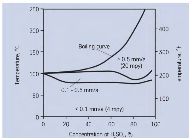
Fig. 2 – Isocorrosion diagram of Nicrofer 5716 hMoW-alloy C-276 in lightly aerated, technical grade sulphuric acid based on immersion test results over at least 120 h.
